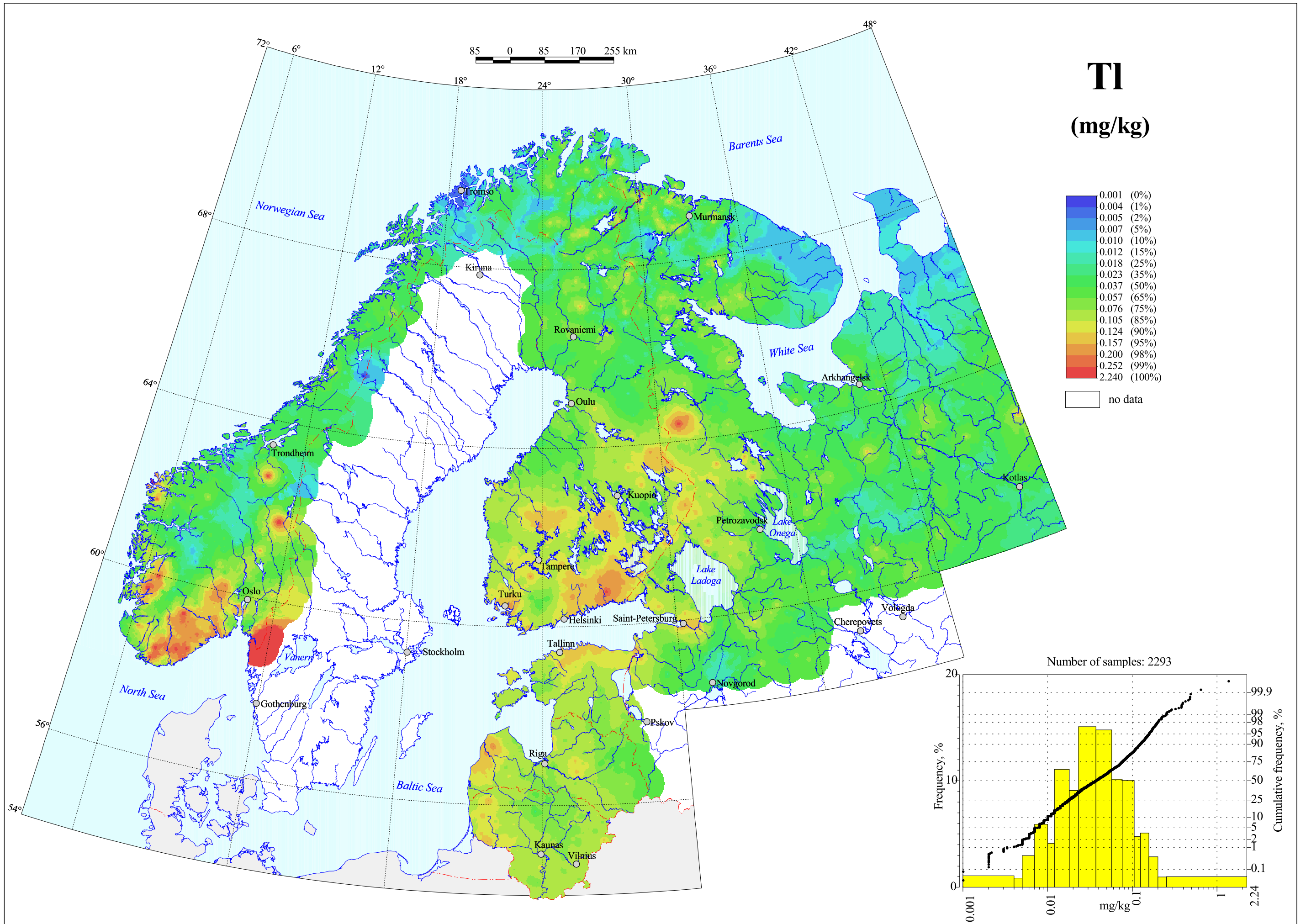
Thallium in Terrestrial Moss, Total Content
